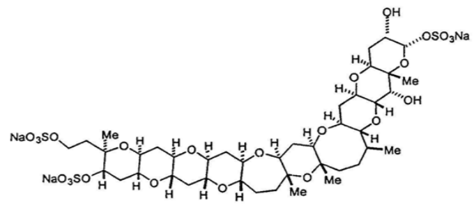
Adriatoxin(ATX)
